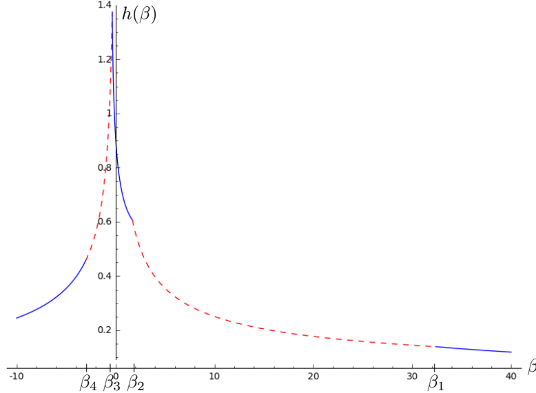
Figure 4.7: Graph of the function h(\beta) , defined in (4.6)
