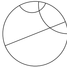
Figure 33.7.7: Hyperbolic geodesics
