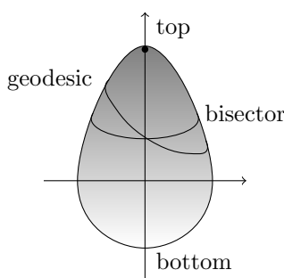
Figure 37.9.14: Egg of revolution
