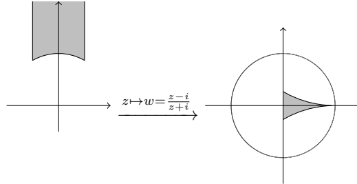
Figure 35.1.7: \sqcup in \mathbf{D}^2
