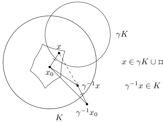
Figure 37.4.21: \sqcap is locally finite and star-shaped
