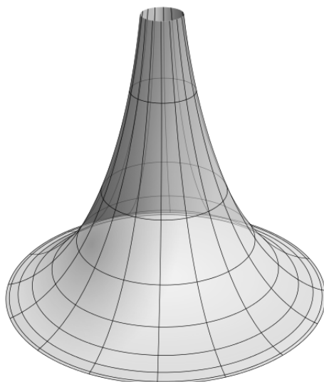
Figure 33.1: Pseudosphere (photo credit: Ermishin Fedor, Creative Commons)
